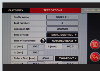
Displacement-controlled test settings
